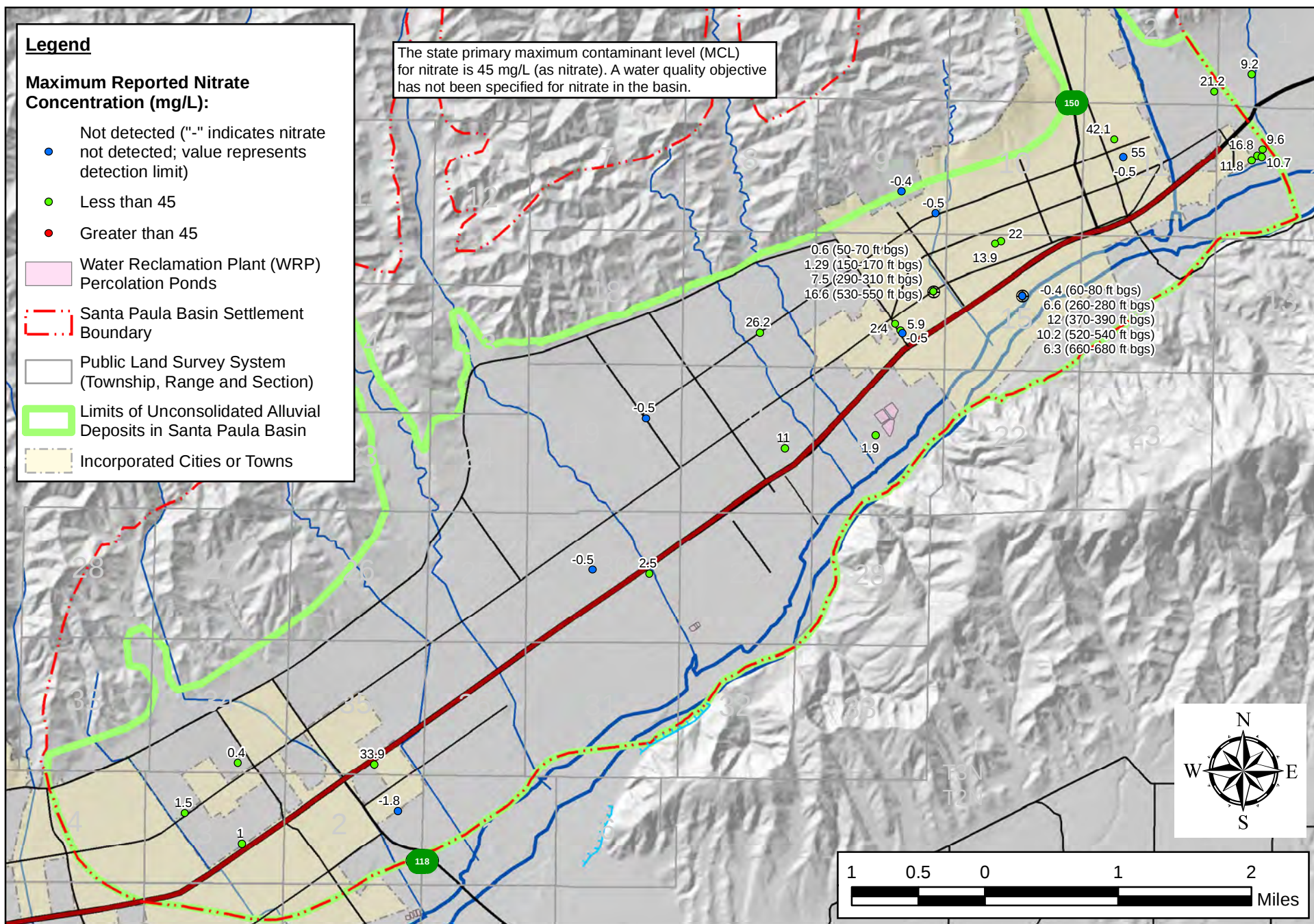
Figure 18. Maximum Reported Nitrate Concentrations in Groundwater, CY 2016
