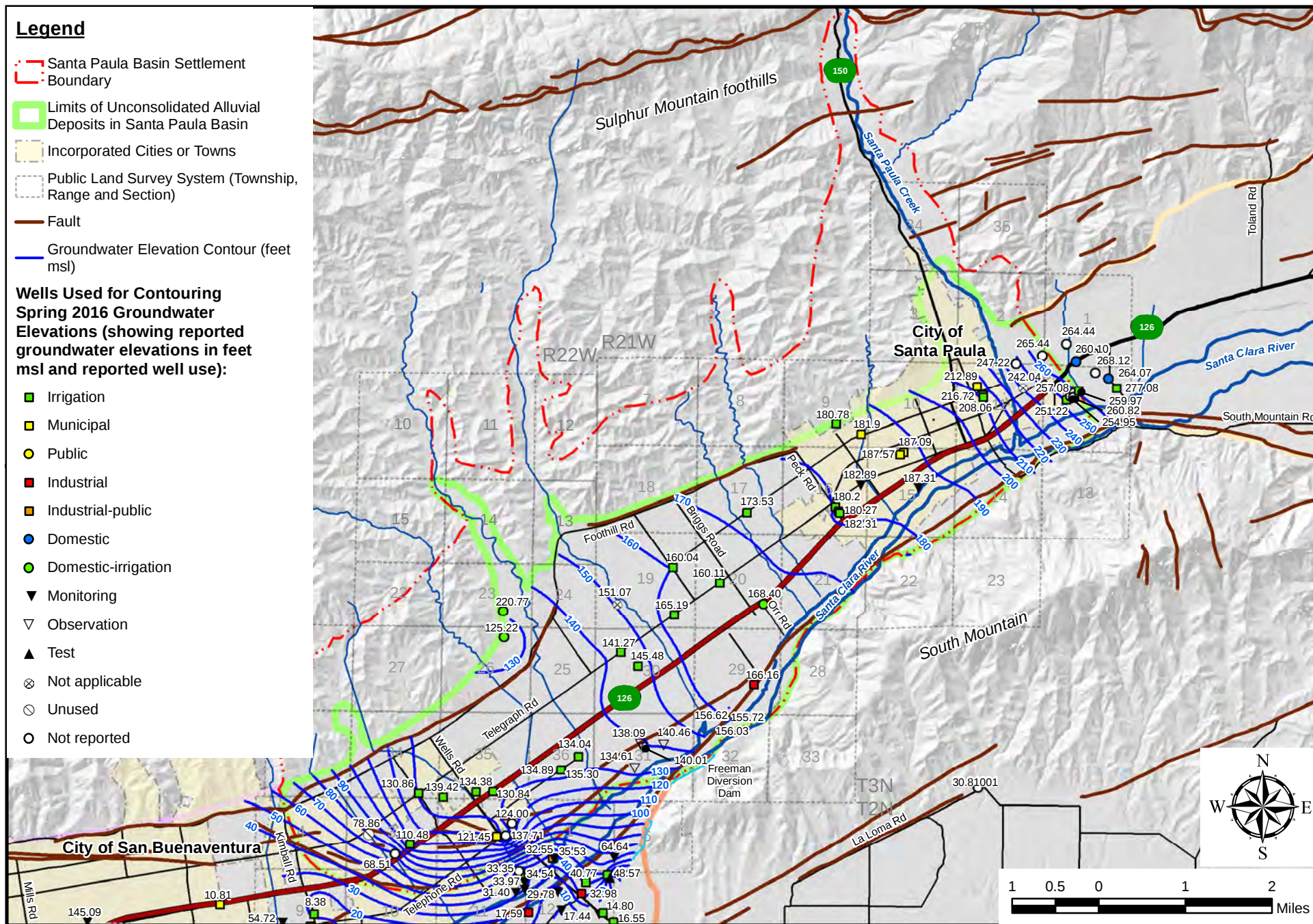
Figure 14. Santa Paula Basin Groundwater Elevation Contours, Spring 2016
