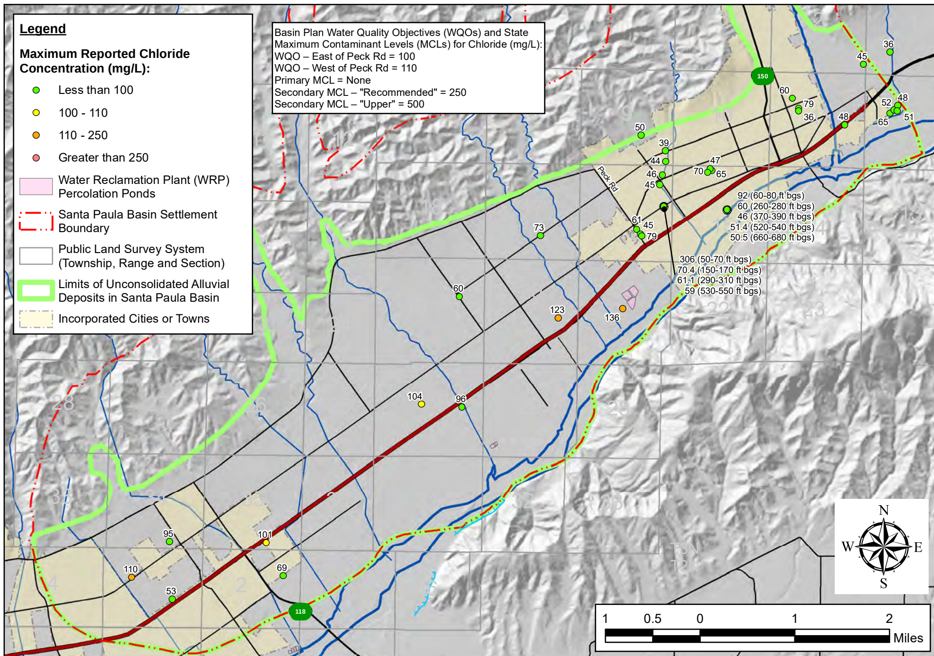
Figure 19. Maximum Reported Chloride Concentrations in Groundwater, CY 2016
