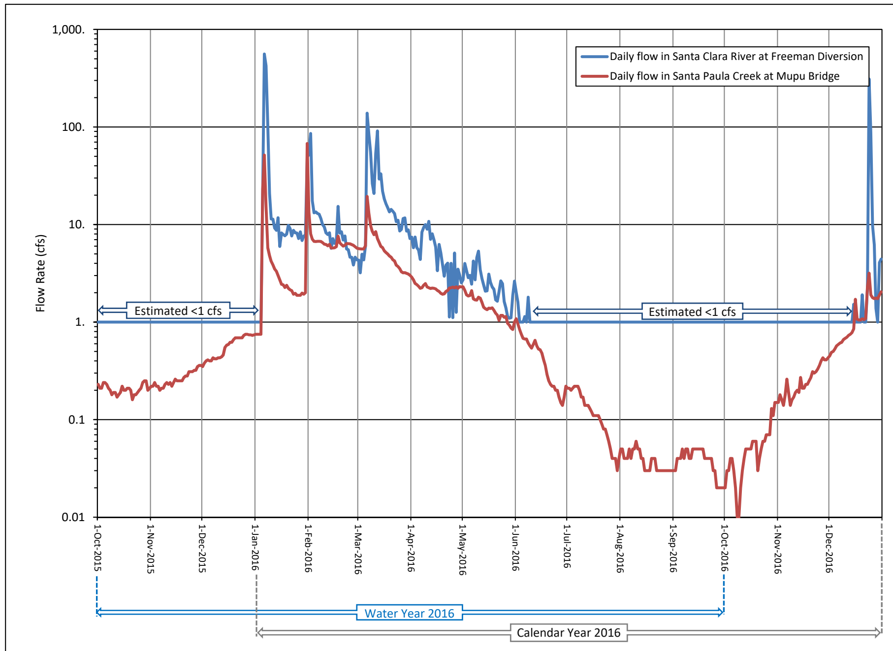
Figure 7. Daily Streamflow in Santa Paula Creek and Santa Clara River, WY and CY 2016
